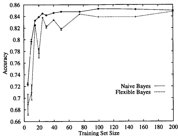
Figure 4: Learning curves testing the first hypothesis about behavior when the normality assumption holds.
