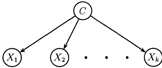
Figure 1: A naive Bayesian classifier depicted as a Bayesian network in which the predictive attributes ( X_1, X_2, \dots, X_k ) are conditionally independent given the class attribute ( C ).
